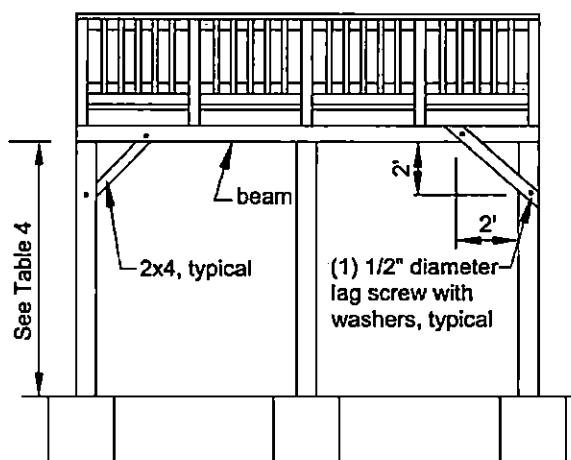
Figure 10. Diagonal Bracing.
